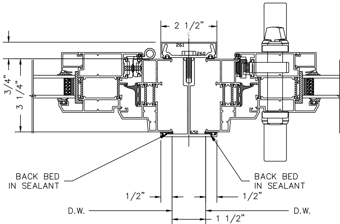
(M2) COMPRESSION MULL DETAIL SCALE: 3/8" = 1"
