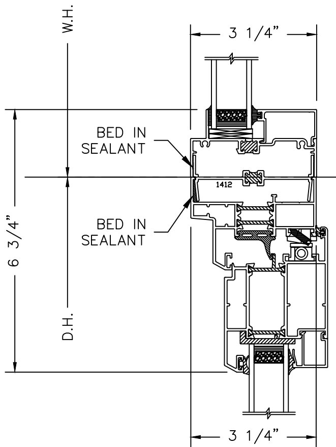
(M1) STACK MULL DETAIL SCALE: 3/8" = 1"
